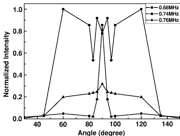
FIG. 6. Measured far-field radiation patterns for various frequencies vs angle.
